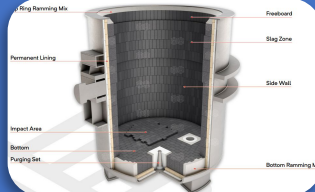
Tundish Refractory
